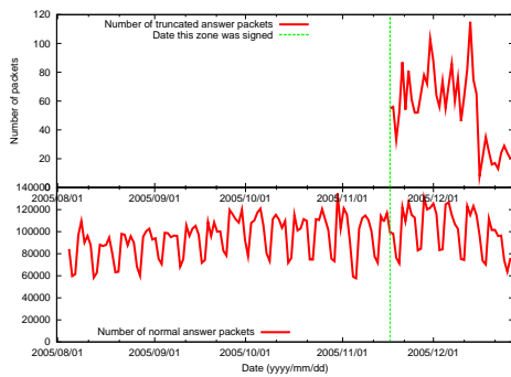
Figure 16: 195.in-addr.arpa
