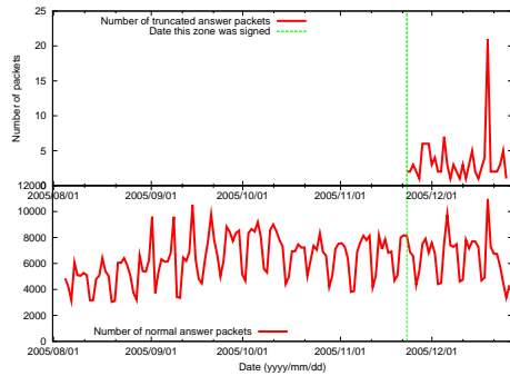
Figure 14: 145.in-addr.arpa
