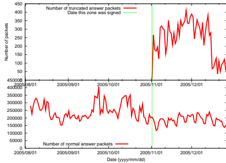
Figure 18: 213.in-addr.arpa
