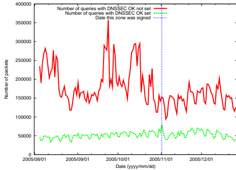
Figure 7: 213.in-addr.arpa
