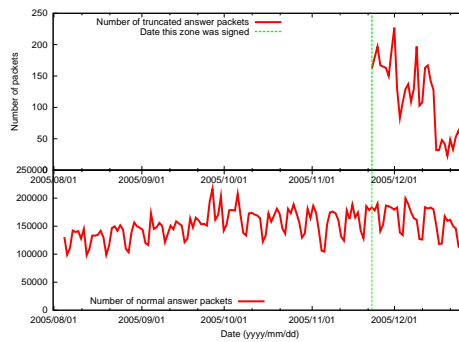
Figure 17: 212.in-addr.arpa
