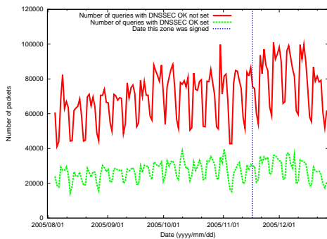
Figure 5: 195.in-addr.arpa
