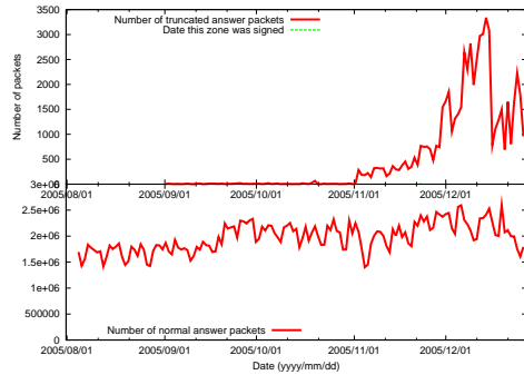
Figure 12: All zones
