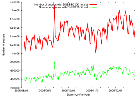
Figure 1: All zones
