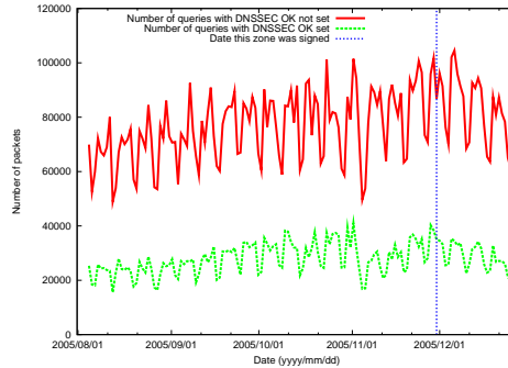
Figure 8: 217.in-addr.arpa
