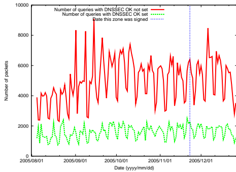
Figure 3: 145.in-addr.arpa
