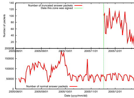
Figure 15: 193.in-addr.arpa
