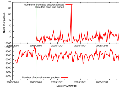
Figure 13: ripe.net
