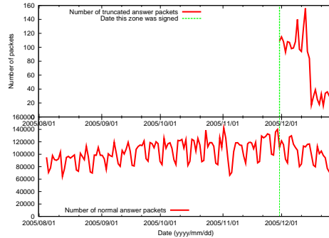
Figure 19: 217.in-addr.arpa
